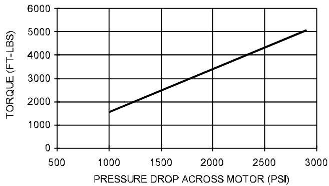
DIGGER TORQUE
