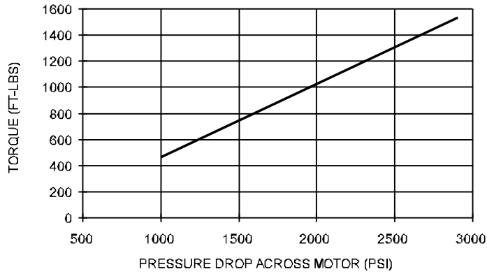
DIGGER TORQUE
