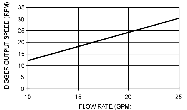
DIGGER SPEED
