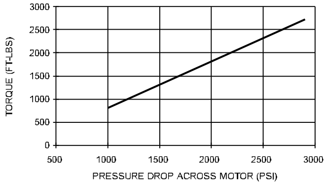
DIGGER TORQUE
