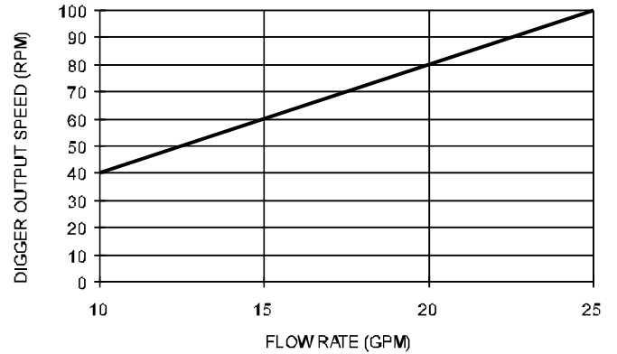
DIGGER SPEED
