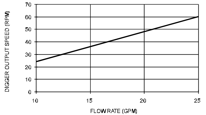
DIGGER SPEED
